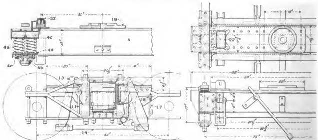
Figs. 4311-4314. Barber Tender Truck. Standard Car Truck Co.
